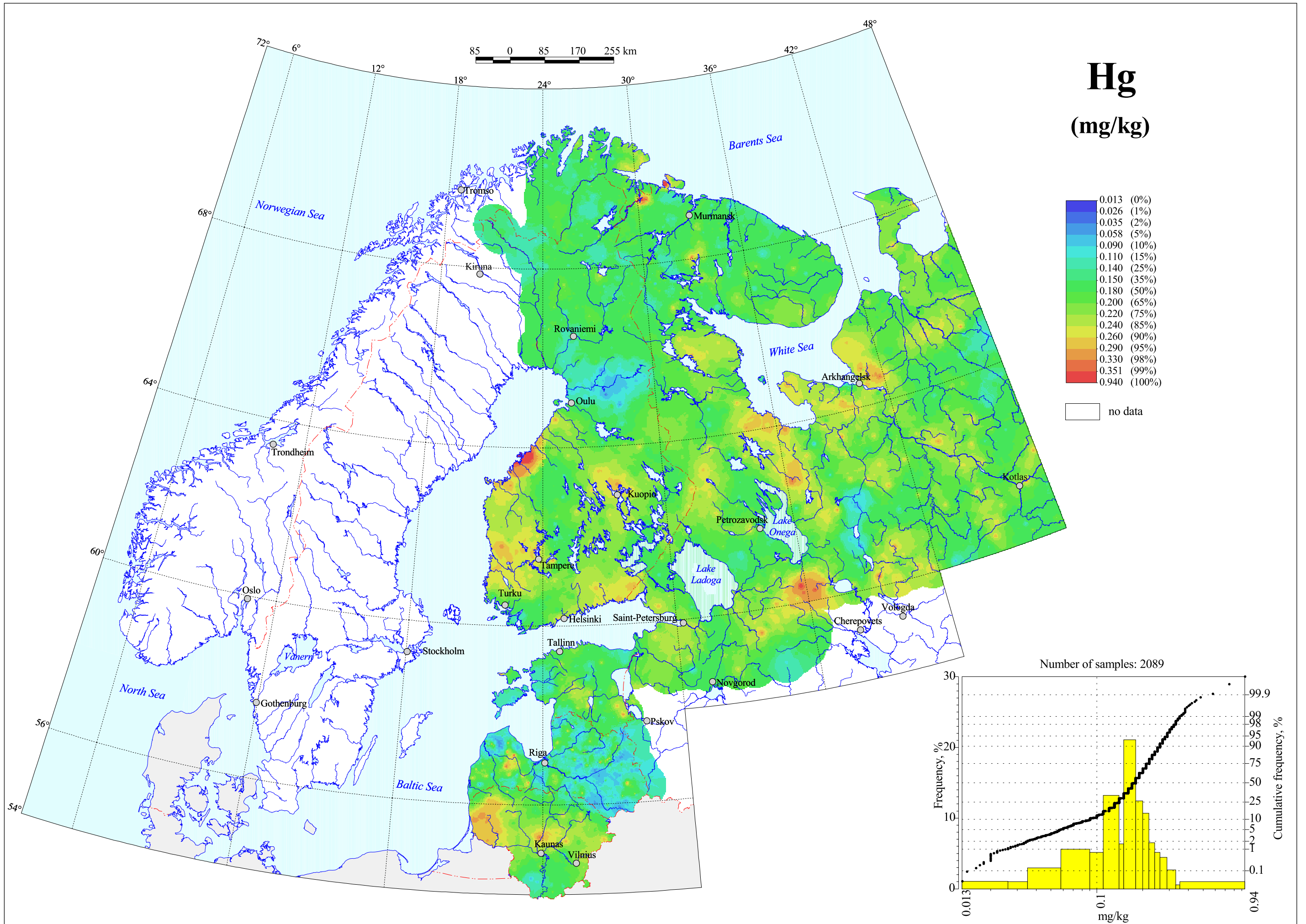
Mercury in Organic Soil Layer, Total Content
